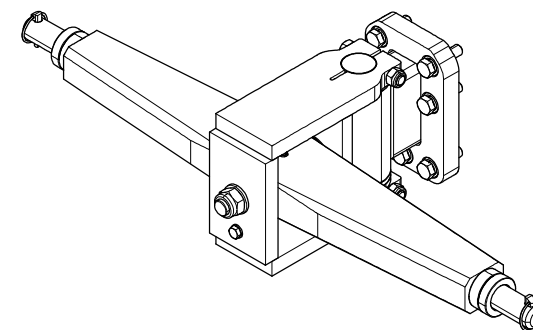
Tazne pravitko, uchyceni II. kat., èep III kat. Standard towing bracket, attachment II. cat., Pin III. cat.
