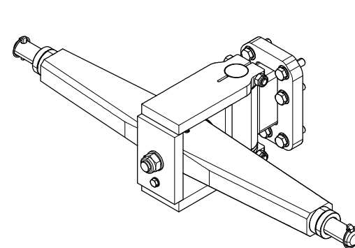
Tazne pravitko, uchyceni II. kat., cep III kat. Standard towing bracket, attachment II. cat., Pin III. cat.
