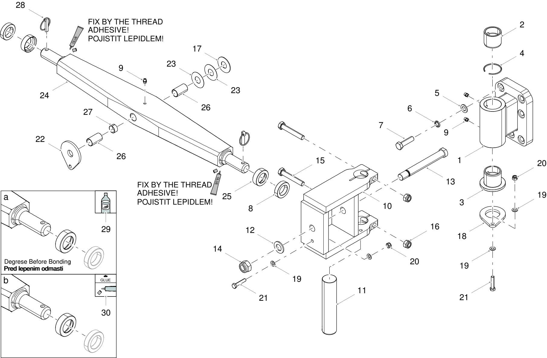
Towing Bracket B
