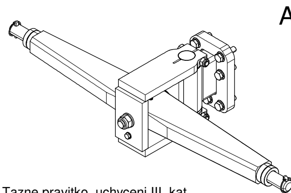
Tazne pravitko, uchyceni III. kat Standard towing bracket, attachment III. cat.
