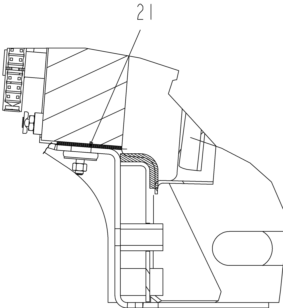
DETAIL B SECTION D-D
